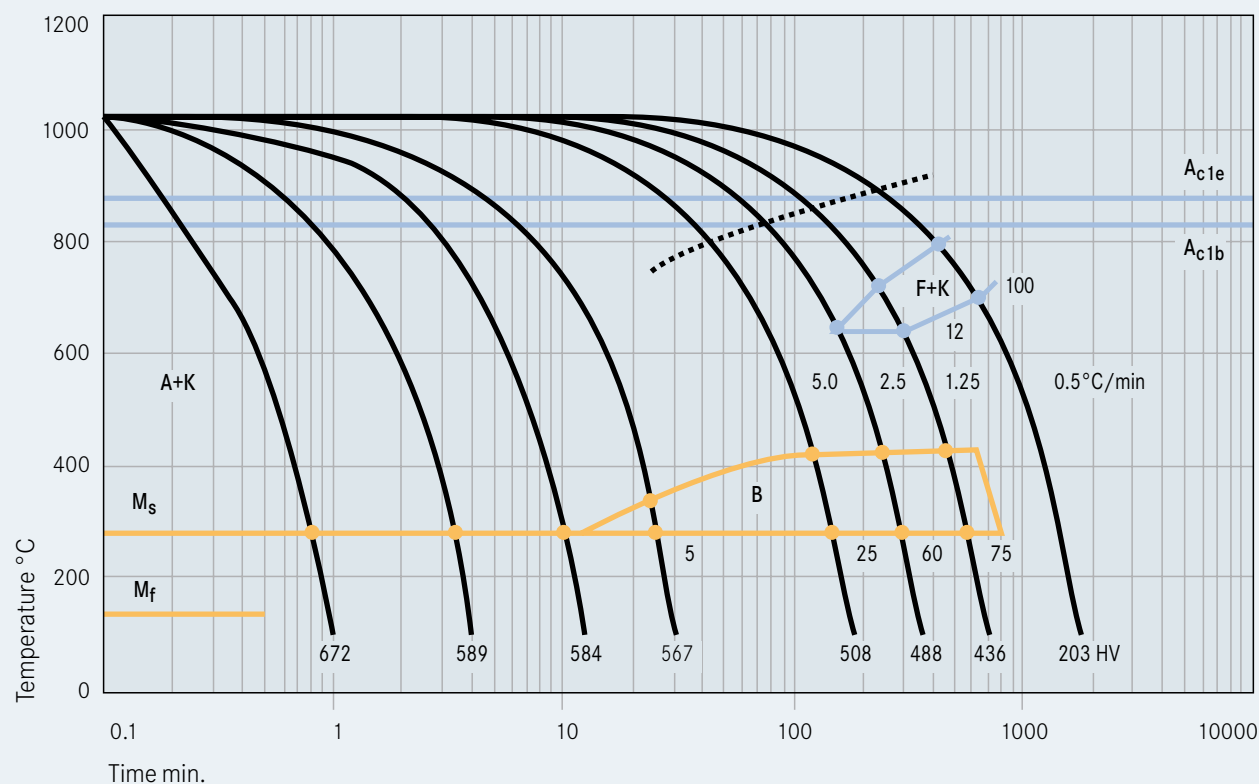
TTT-Diagram Austenitizing temperature 1020 °C
