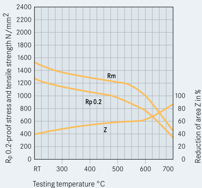
Diagram of high temperature strength 30 mm Ø, 1020°C Oil
