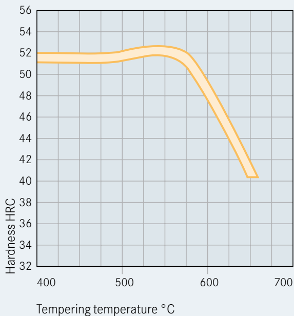
Tempering diagram 60 mm Ø, 1020°C Oil
