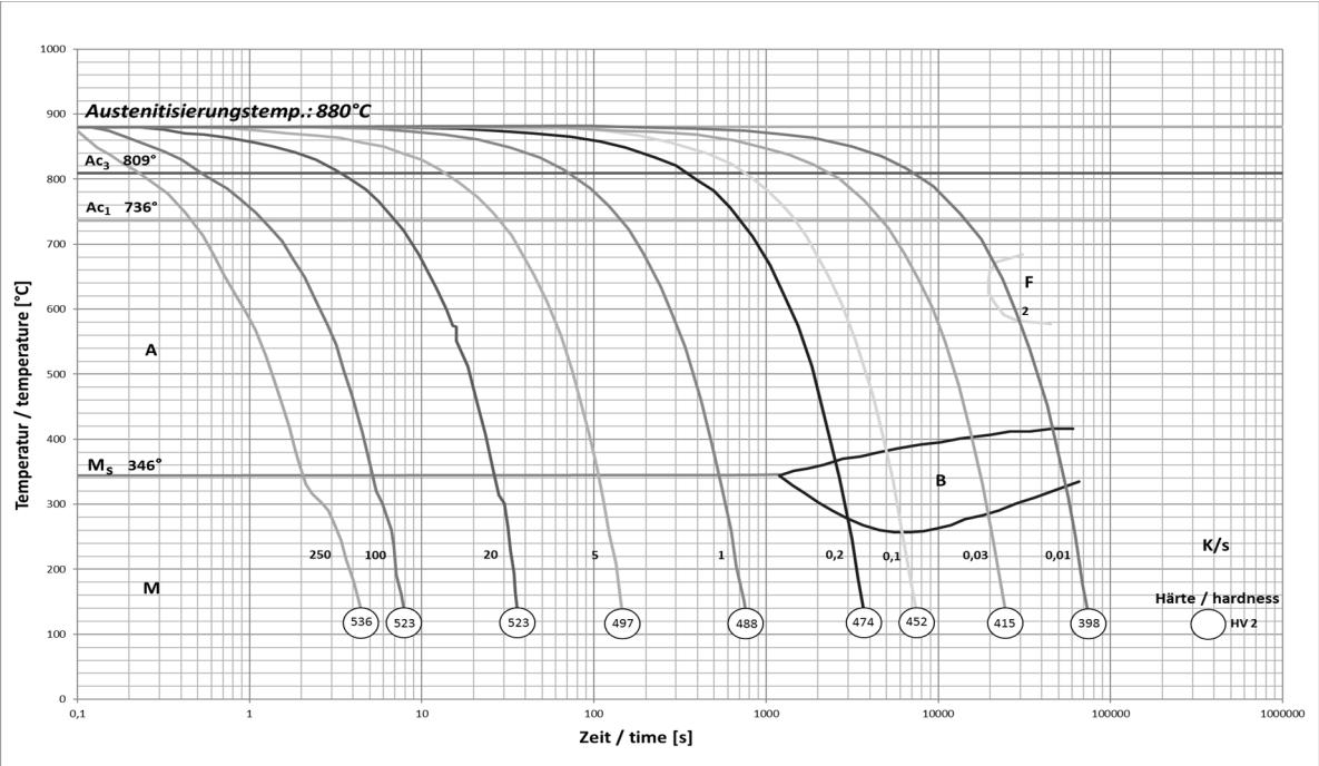
CCT-diagram
